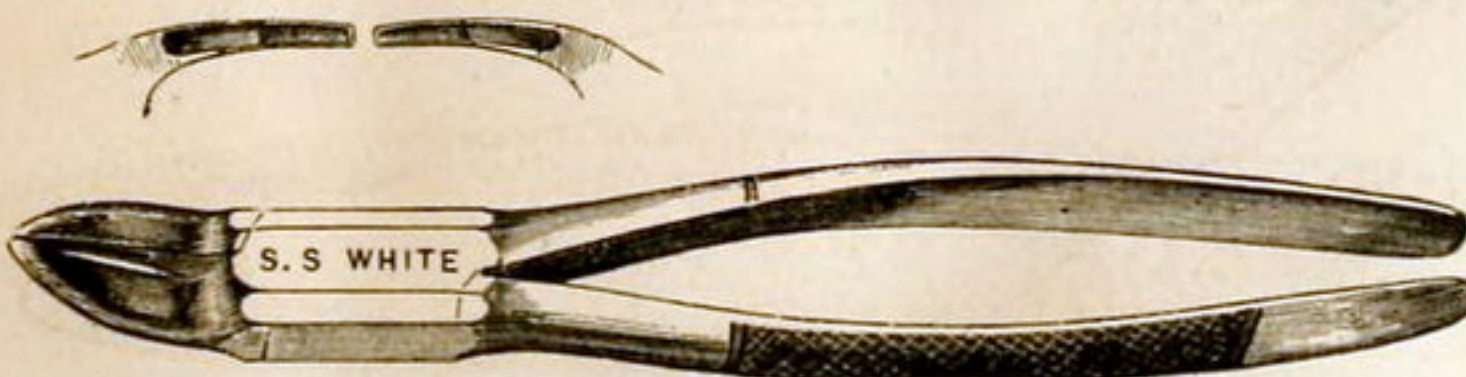
No. 36—Half Curved, Narrow Beak for crowded Teeth.
